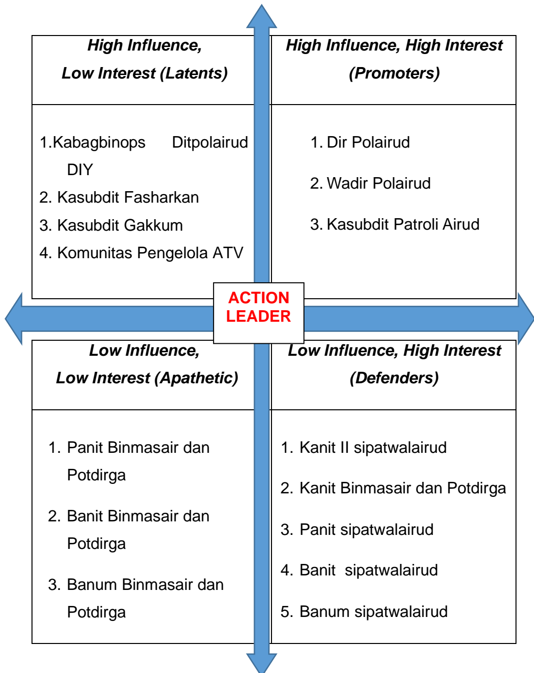
Gambar 2.1. Kuadran stakeholder
