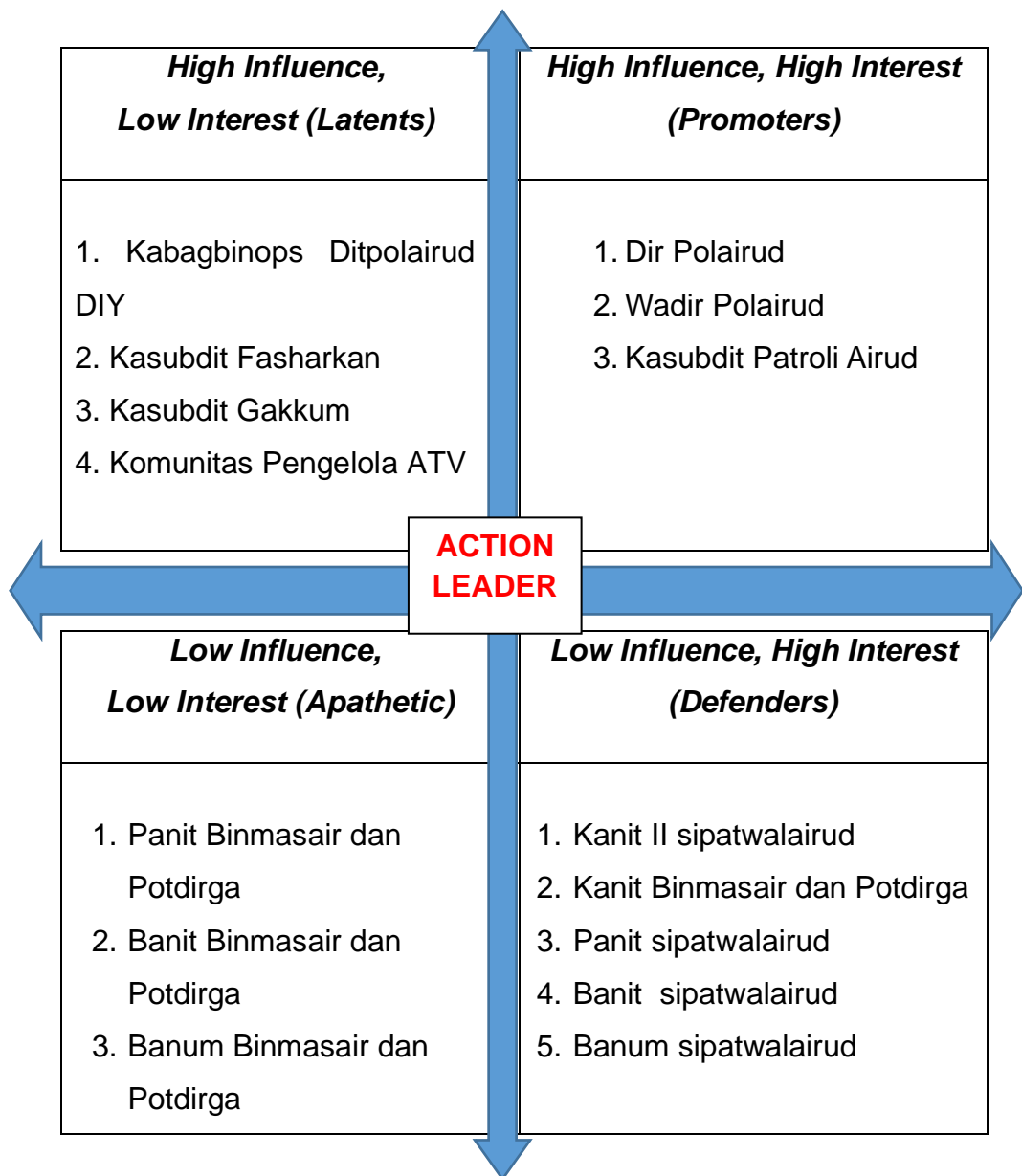
Gambar 4.3 Kuadran Stakeholders
